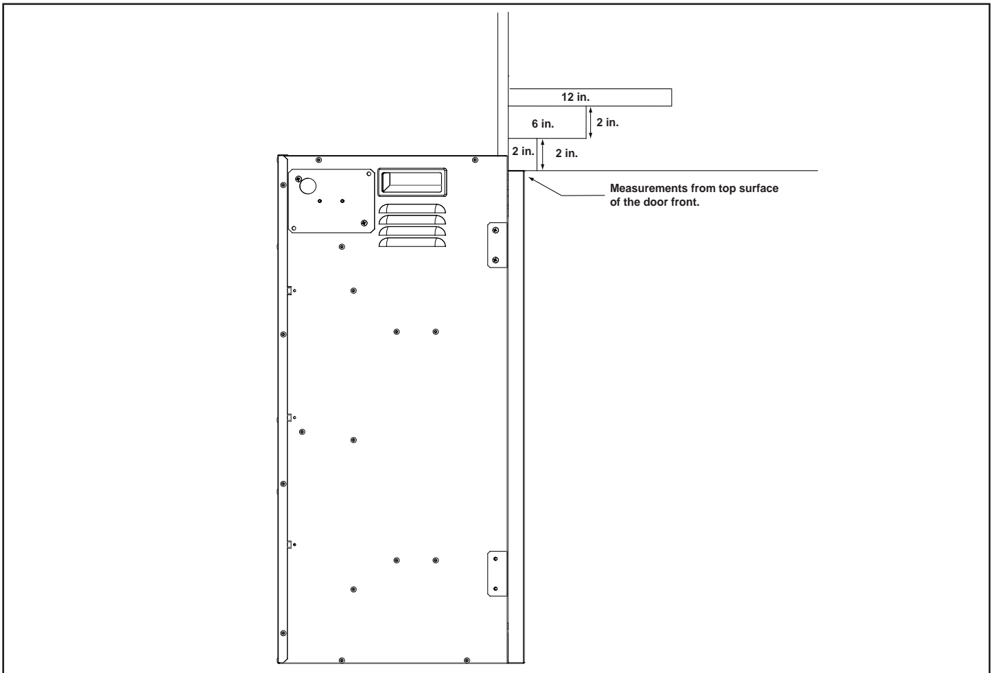
Figure 3.1 Minimum Vertical and Maximum Horizontal Dimensions of Combustible Mantels.
