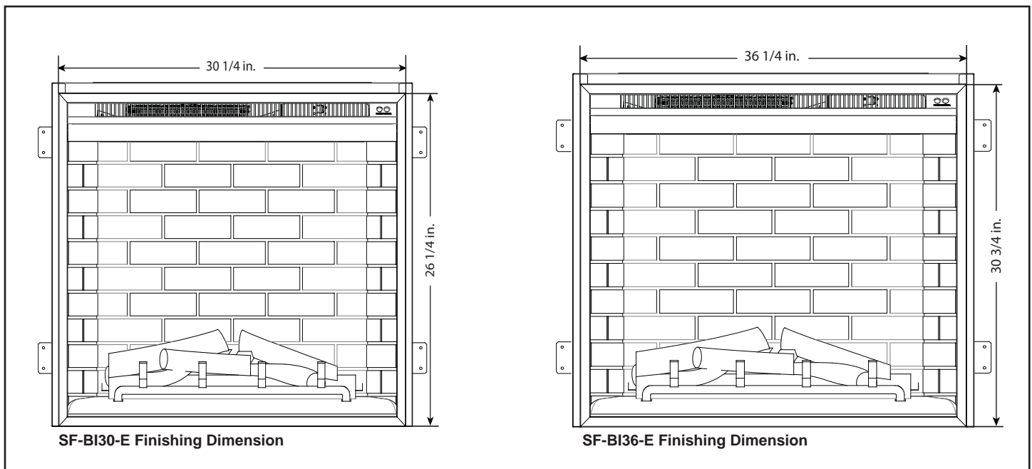
Figure 4.4 Finishing Dimensions
