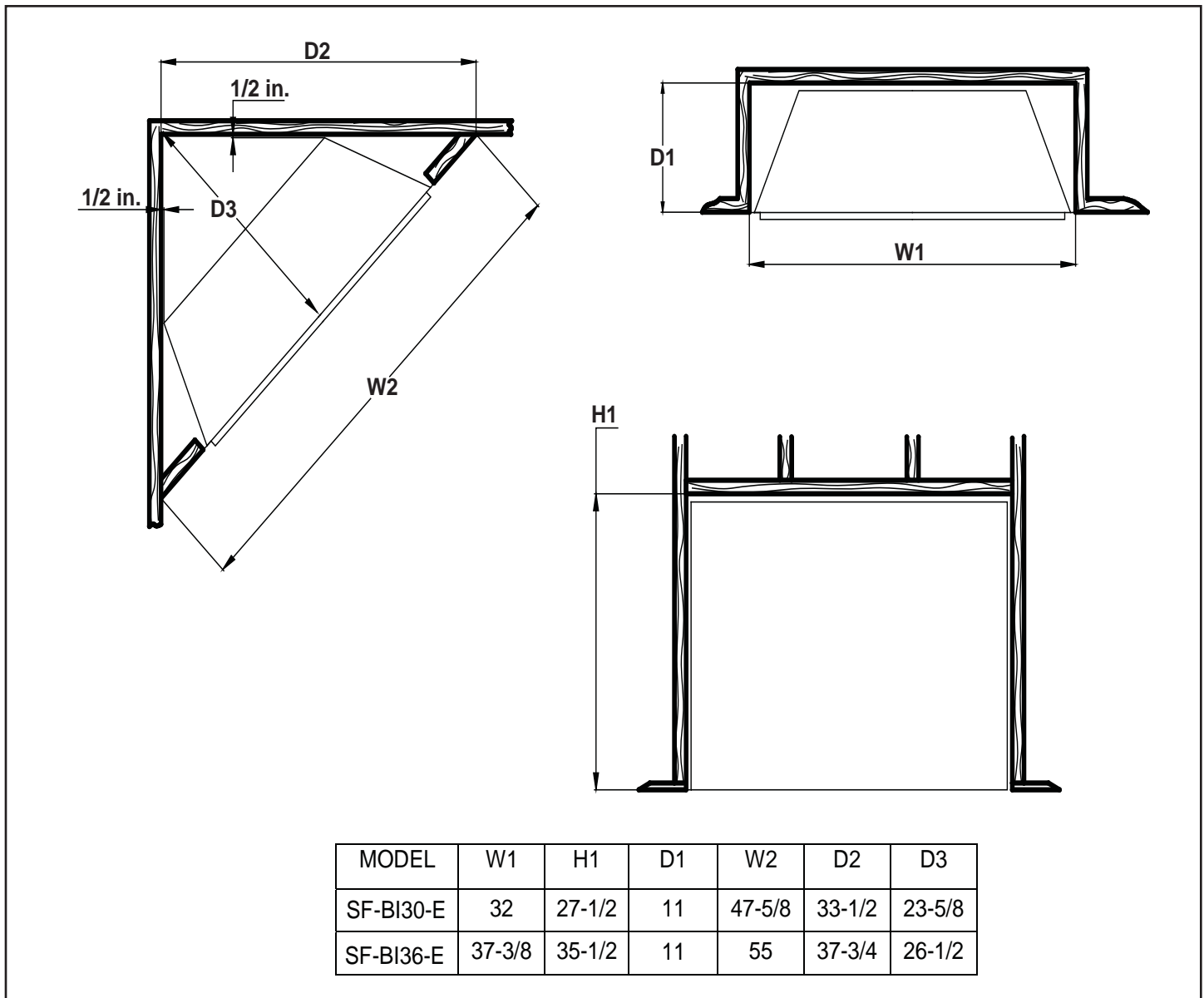
Figure 4.1 Clearance Requirements
