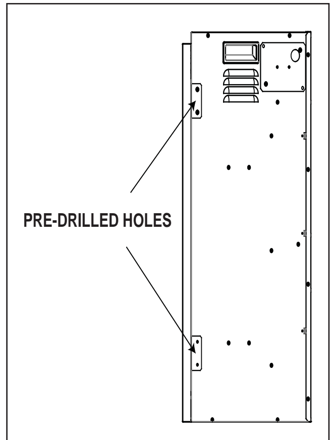
Figure 4.2 Pre-drilled Hole Location
