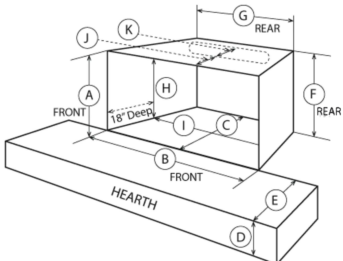
Fireplace Dimensions
